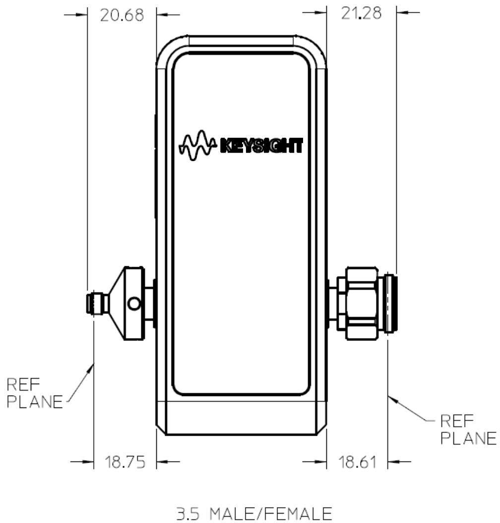
Figure 5-23 N4691D Modules (2-Port) – 3.5 mm Male/Female
