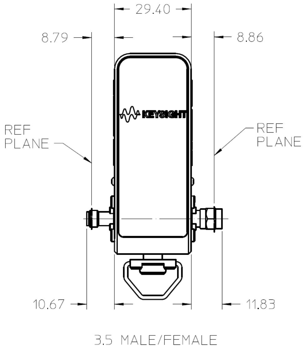
Figure 5-14 N7555A Modules (2-Port) – 3.5 mm Male/Female
