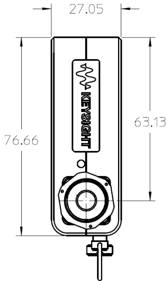
Figure 5-15 N755xA Modules (2-Port) – Side View
