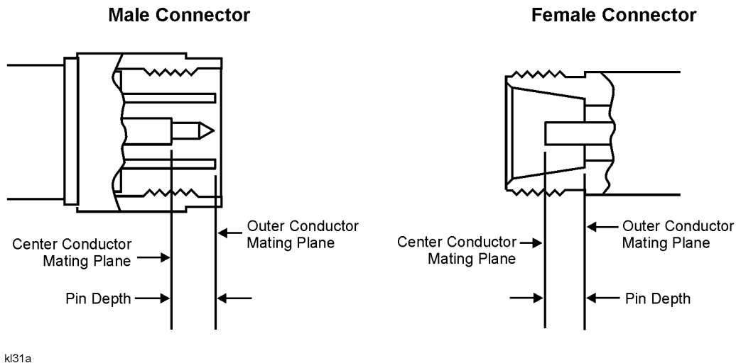
Figure 5-5 Pin Depth for Type-N Connectors
