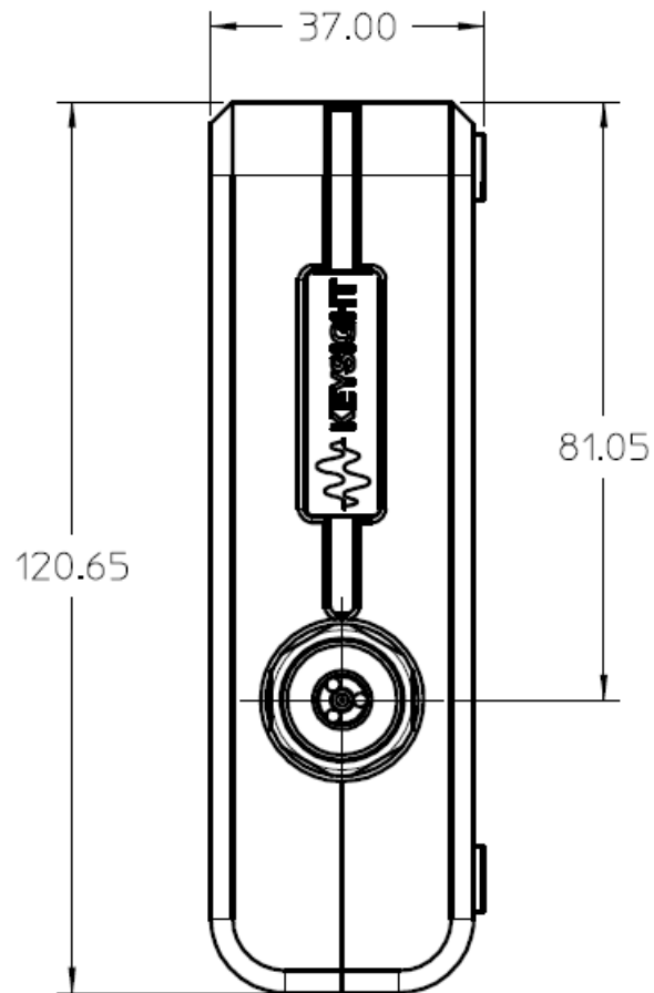
Figure 5-28 N469xD Modules (2-Port) – Side View
