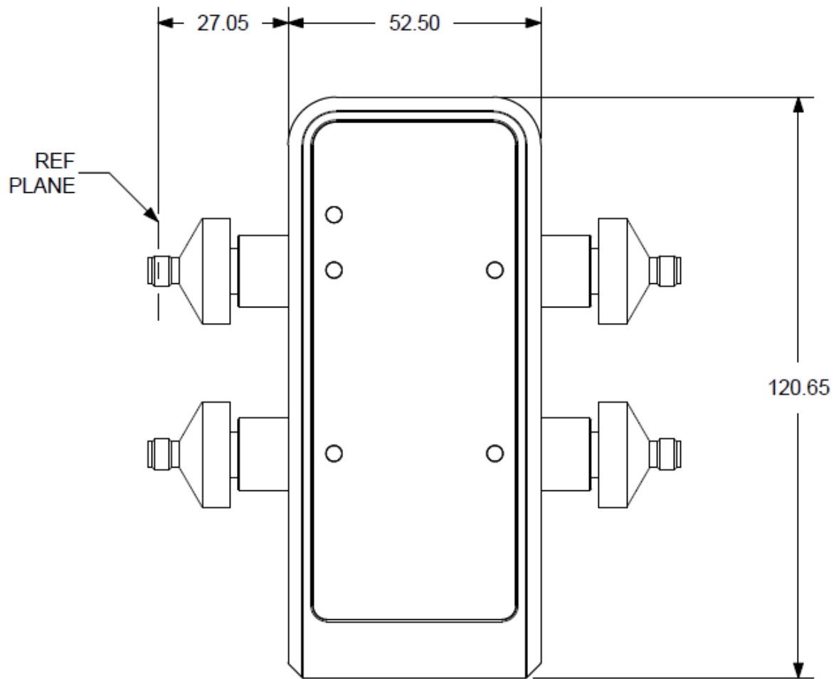
Figure 5-17 N443xD Modules (4-Port) - 3.5 mm Female
