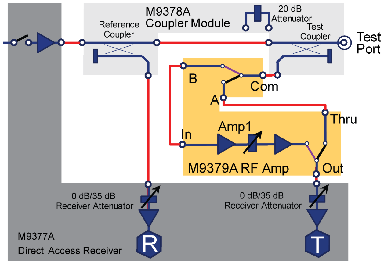
Figure 3. Extending dynamic range of the M9485A PXIe VNA using the M9379A
