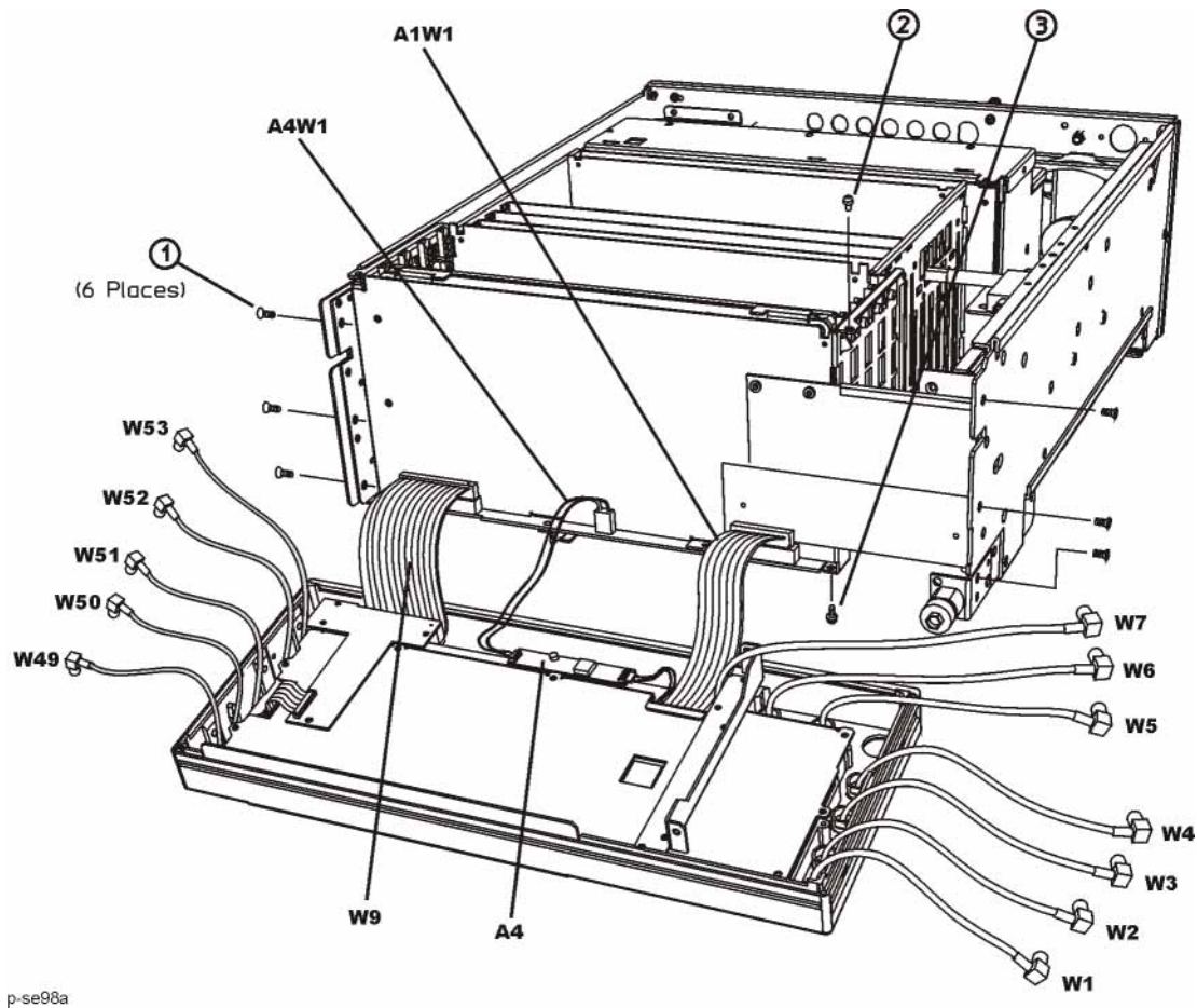
Figure 5 Front Panel Removal
