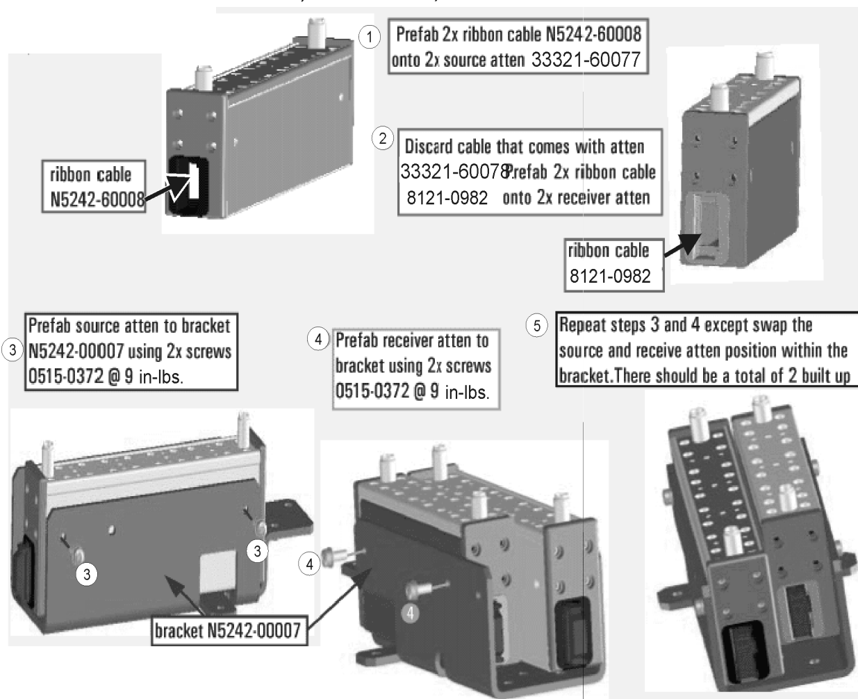
Figure 5 A35, A36 Source Attenuators Assembly and A43, A44 Receiver Attenuators Assembly (0515-0372, 8121-0982, 33321-60077, 33321-60078, N5242-60007, N5242-60008)
