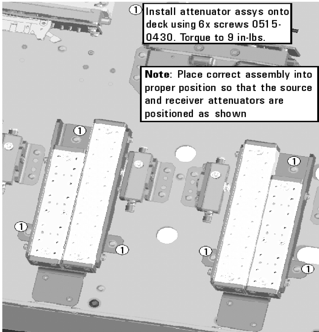
Figure 6 A35, A36 Source Attenuators Assembly and A43, A44 Receiver Attenuators Installation (0515-0430)
