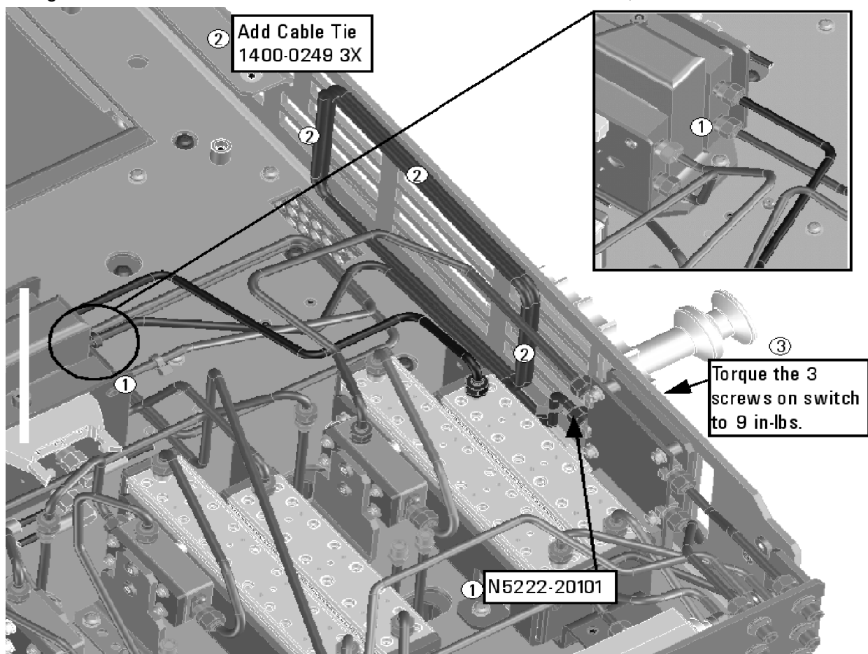
Figure 15 Location of Cable Ties to Secure W48 (1400-0249, N5222-20101)
