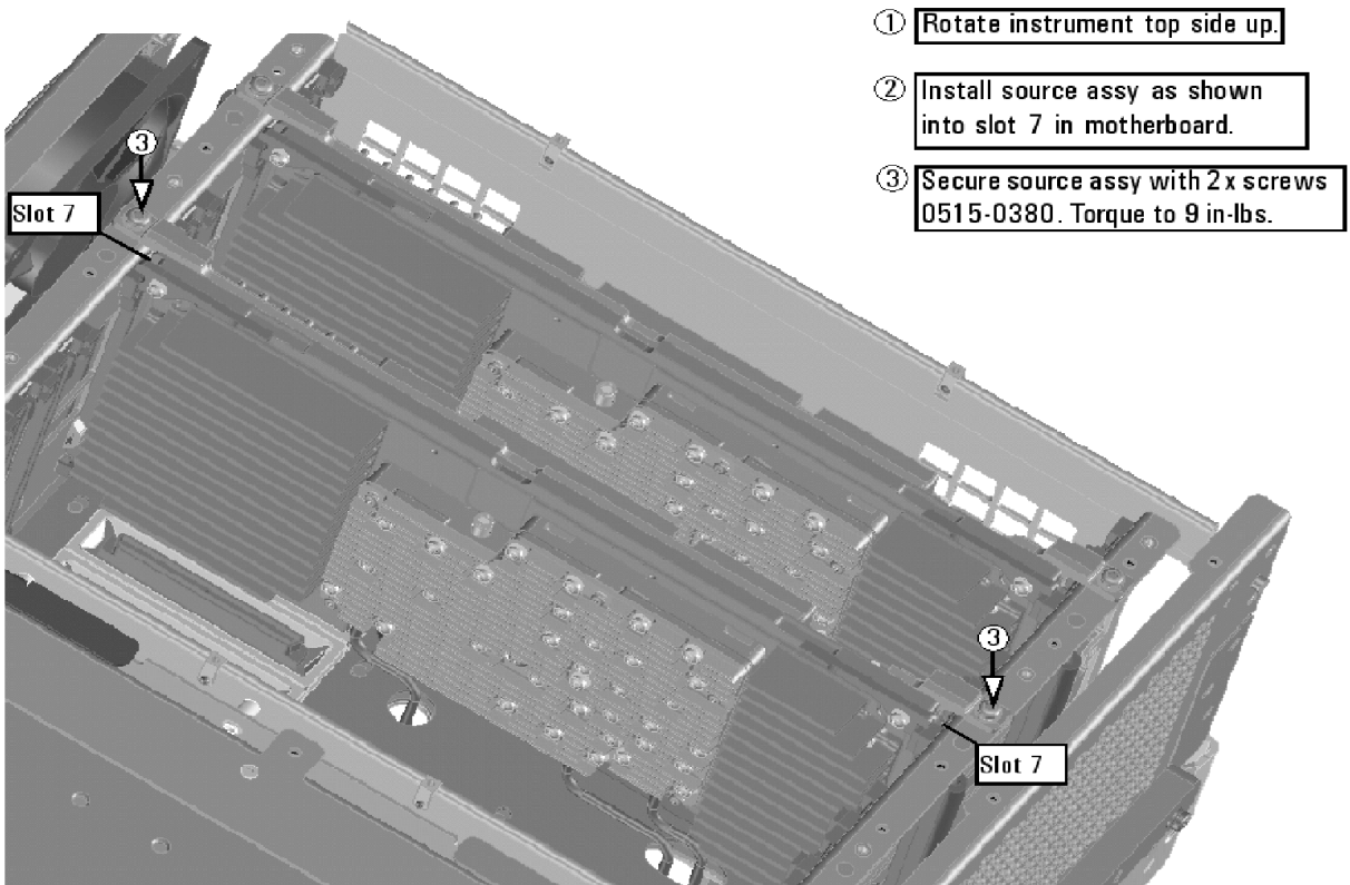
Figure 12 A8 Source 2 Assembly Installation (0515-0380)
