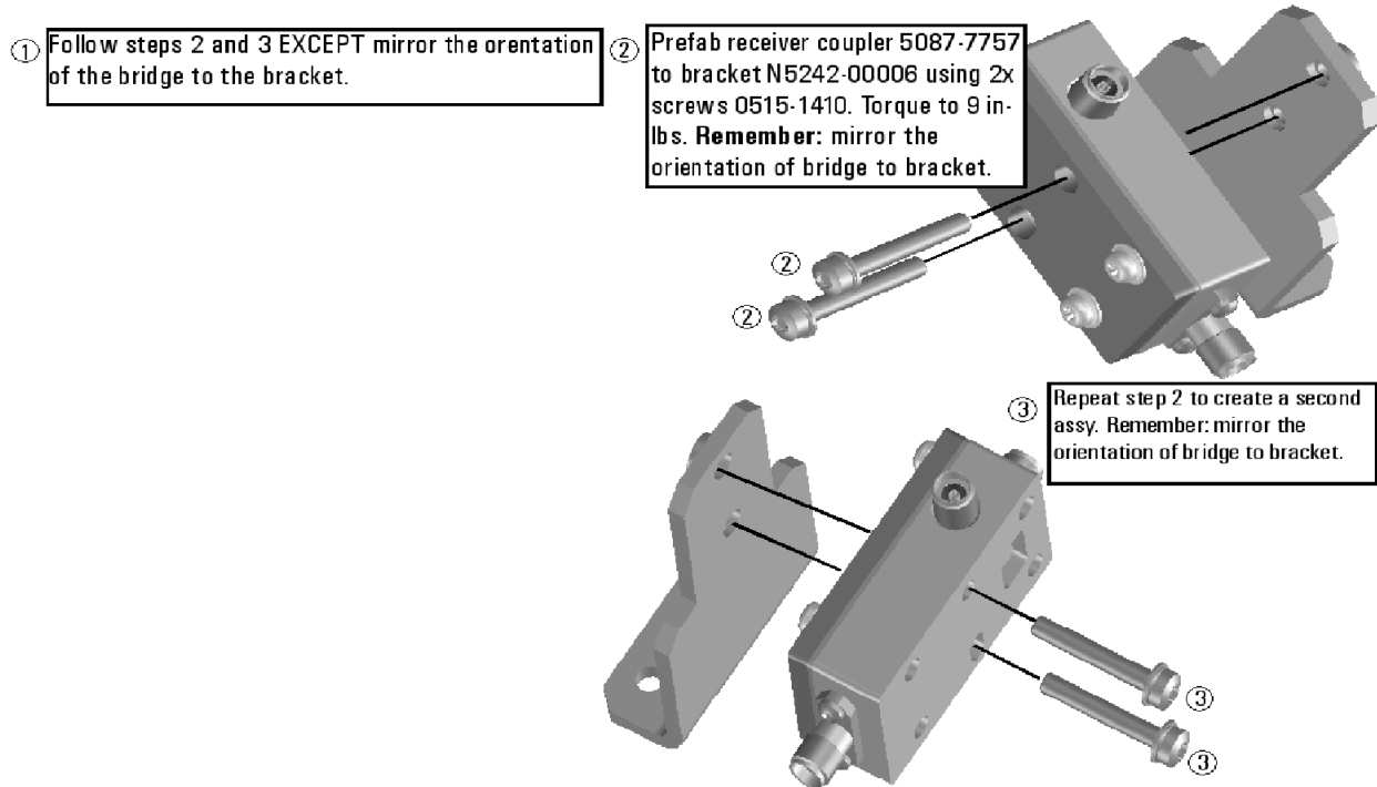
Figure 3 A26 and A27 Receiver Coupler Assemblies (0515-1410, 5087-7757, N5242-00008)
