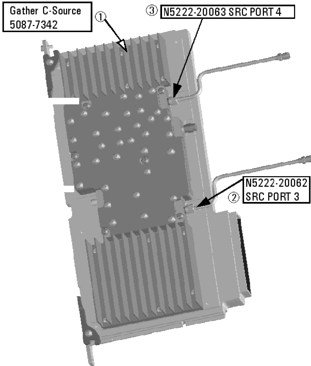
Figure 11 A8 Source 2 Assembly (5087-7342, N5222-20062, N5222-20063)
