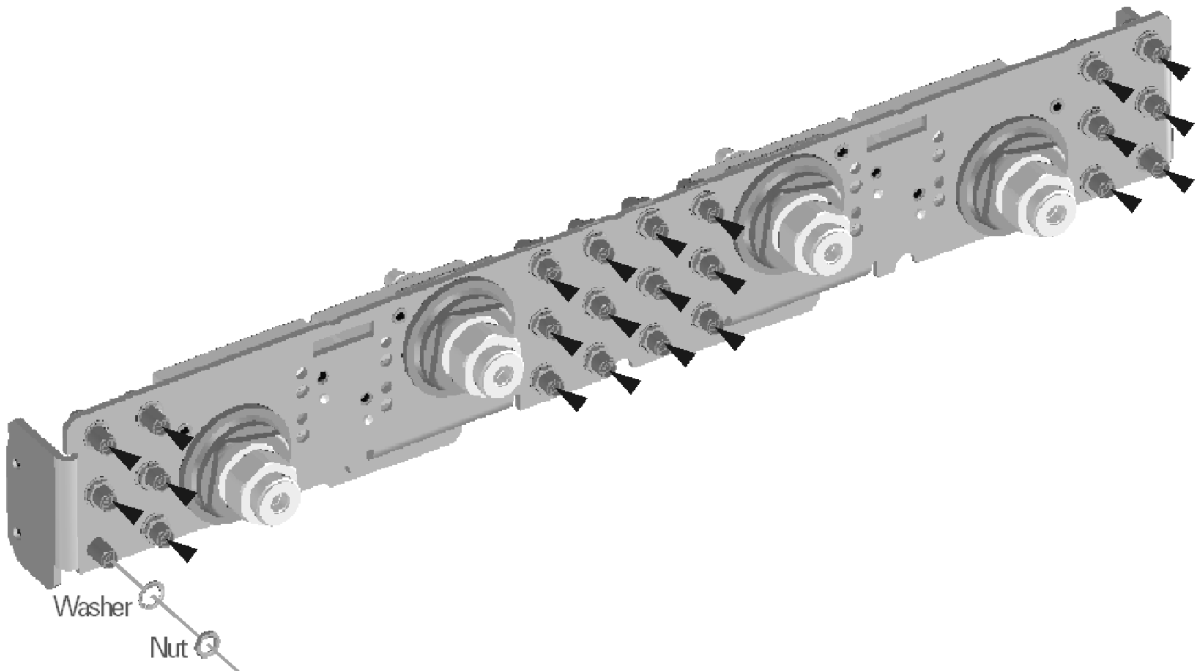
Figure 9 Bulkhead Connectors Installation
