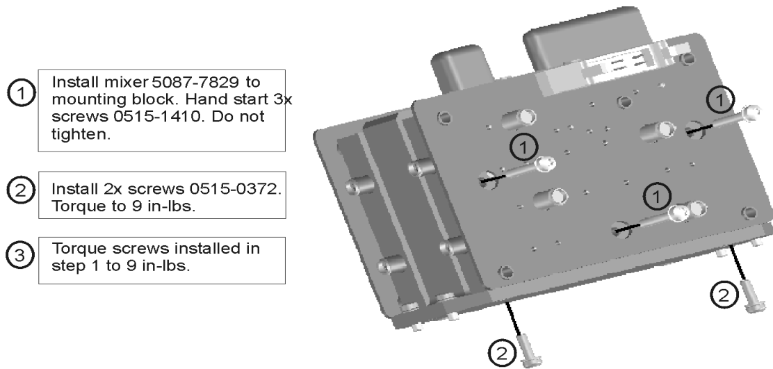
Figure 1 A24 Mixer Brick Assembly (0515-0372, 5087-7829)
