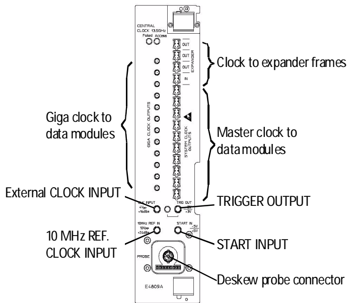
Figure 4 E4809A Clock Module
