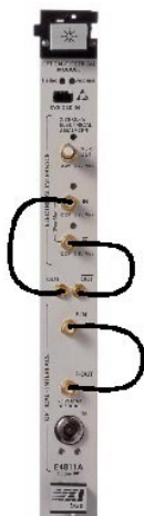
Figure 73 External Connections of an E4811A Module
