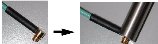
Figure 46 Insert the Cable Connector into the Plug-In Tool
