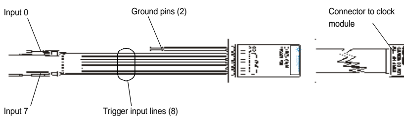
Figure 60 Trigger Input Pod
