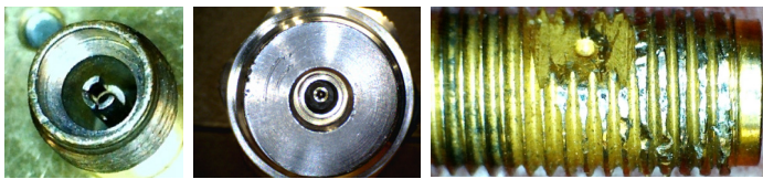
Examples of damaged connectors.
