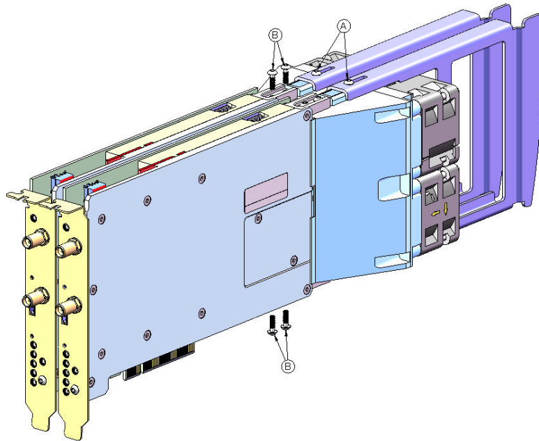
Diagram showing fan/support assembly fixings (U53xxA shown as example).
