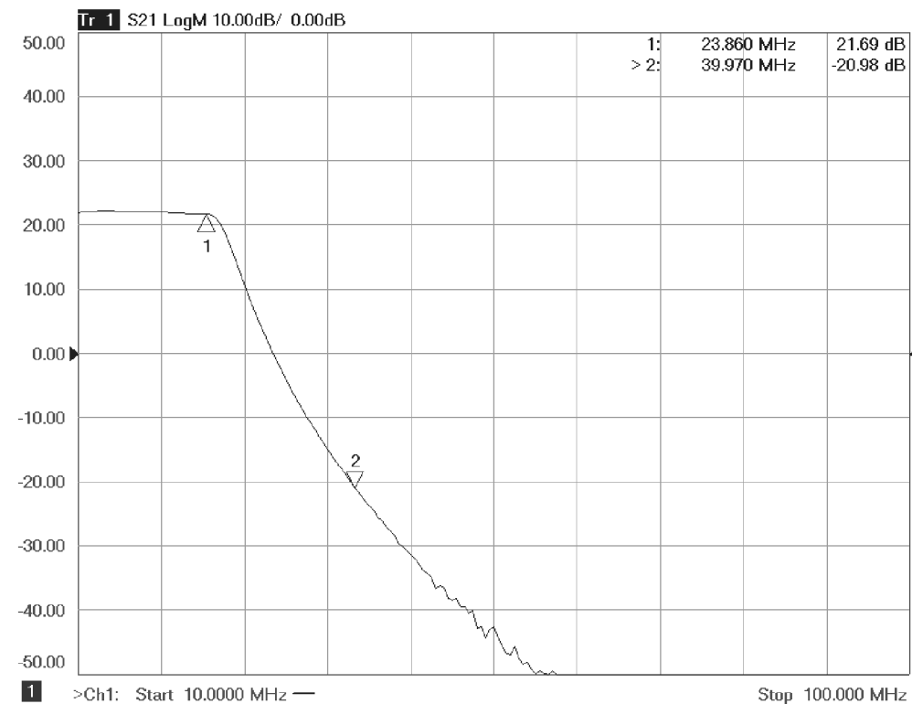
Figure 2-8 Typical IF Gain Response Trace
