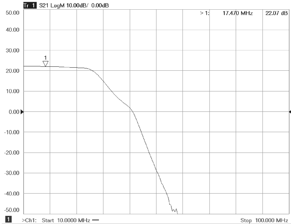
Figure 2-9 Typical Test IF Response Trace
