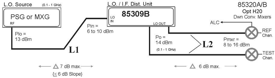
Figure 2-6 Cable Length Configurations (1 of 2)
