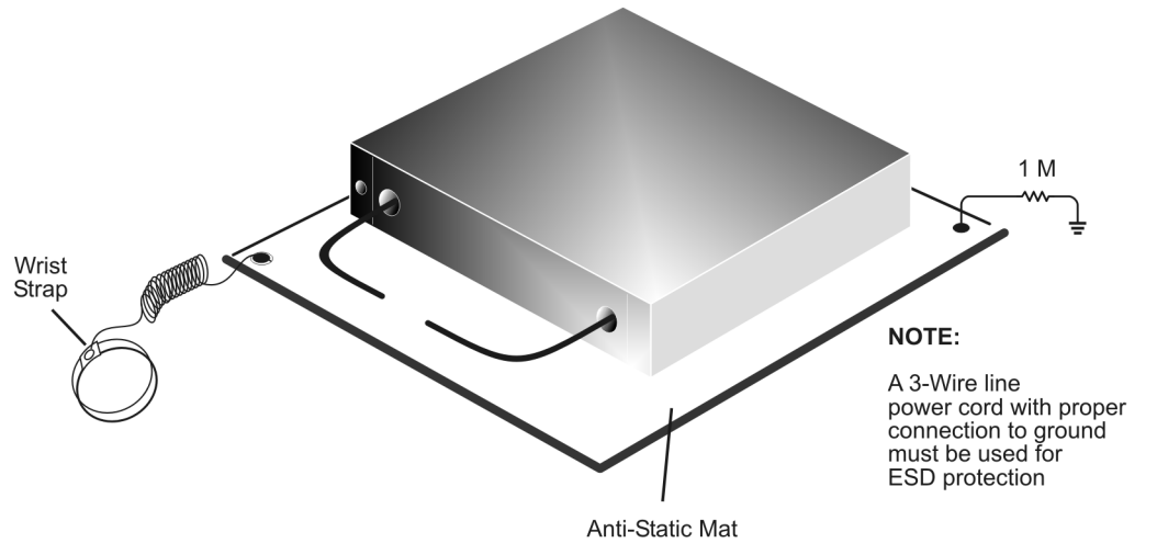
Figure 2-1 ESD Protection Setup
