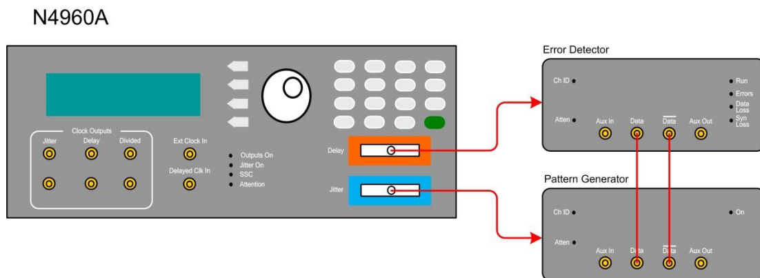
Figure 2. Test Setup
