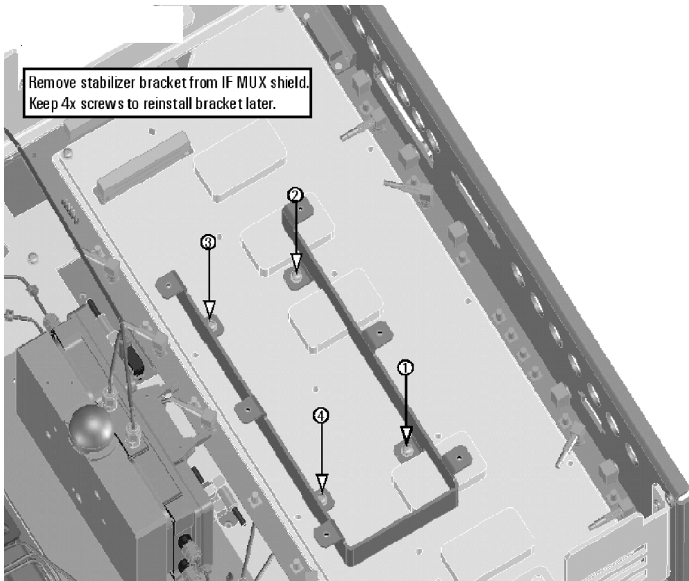
Figure 1 Testset Stabilizer Bracket on A24 IF MUX Board
