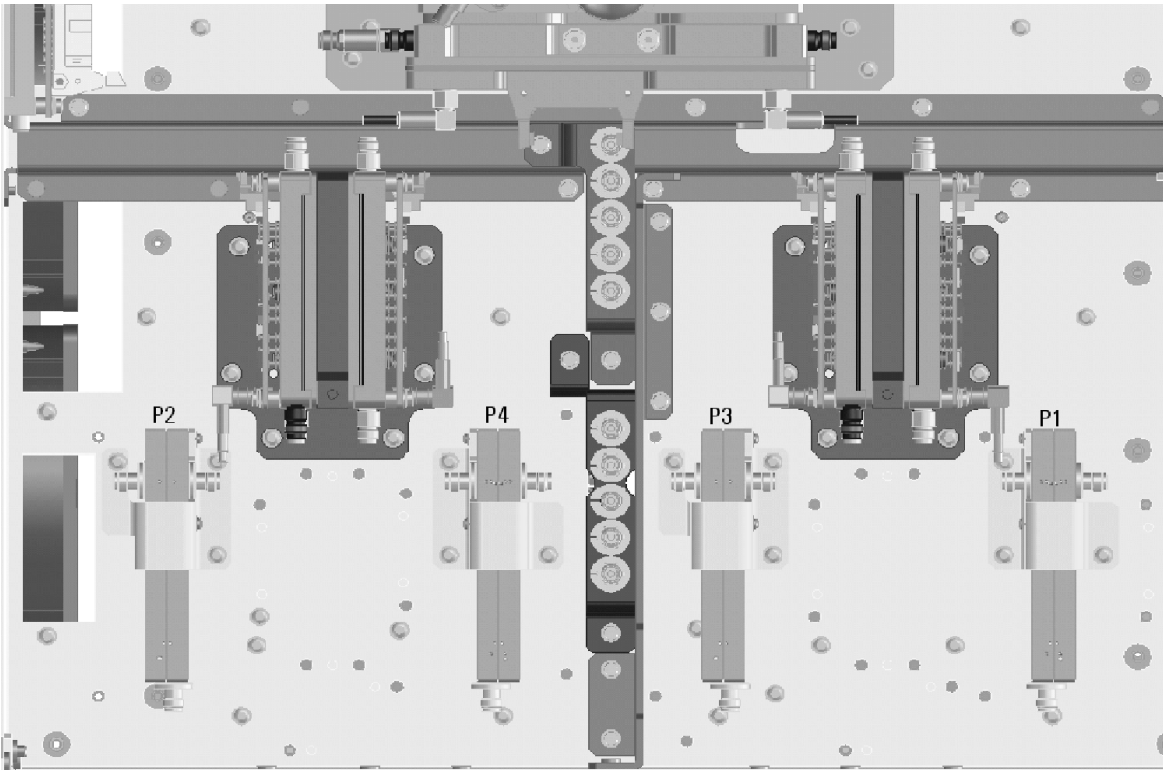
Figure 19 Location of Reference Coupler Assemblies
