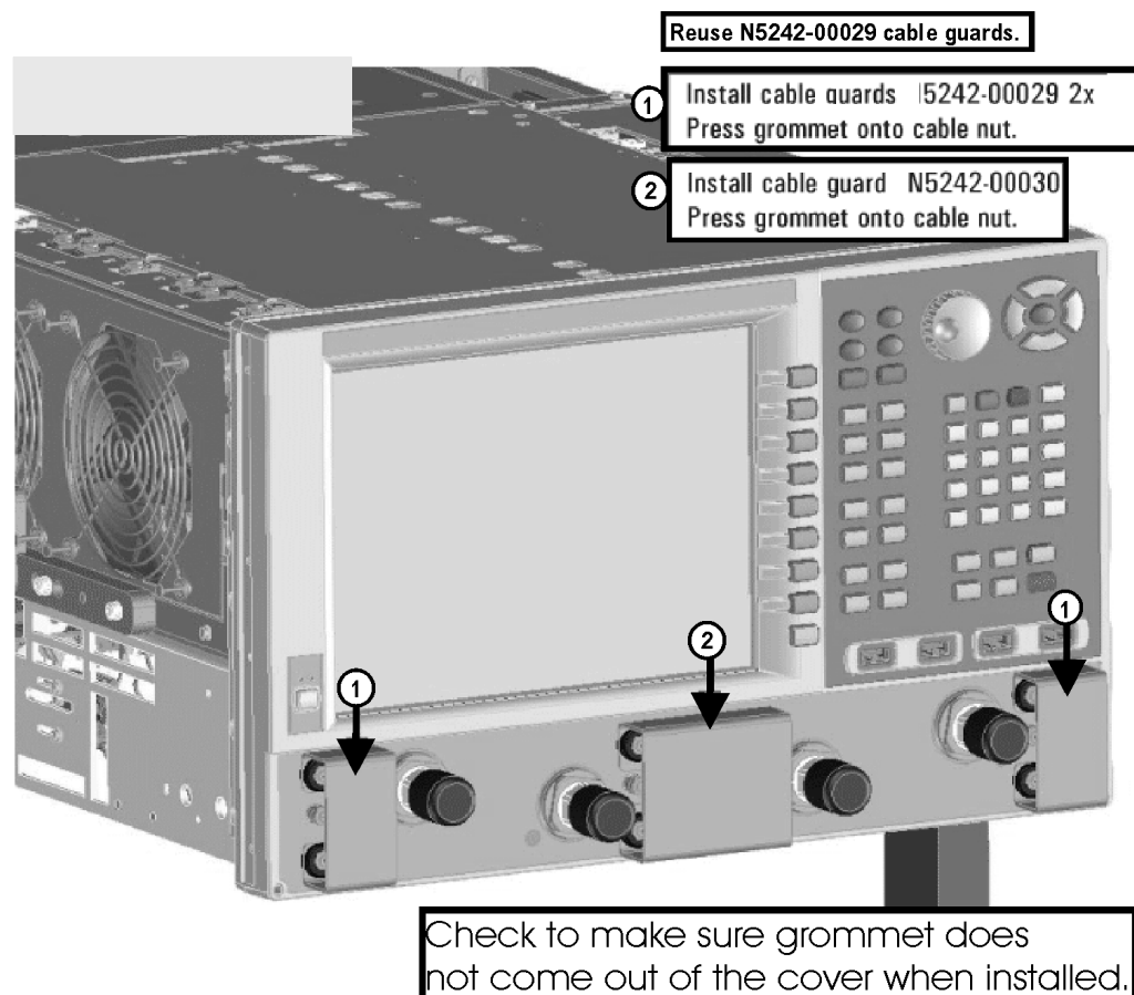
Figure 27 Install the Cable Guards Over the Front Panel Jumpers (N5242-00029, N5242-00030)
