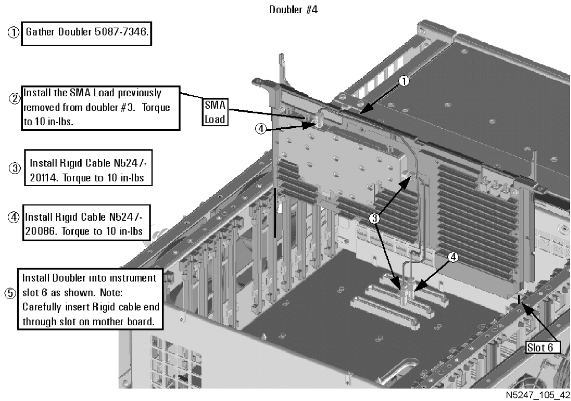
Figure 8 A13 40 GHz Doubler 4 Installation (5087-7346, N5247-20086, N5247-20114)
