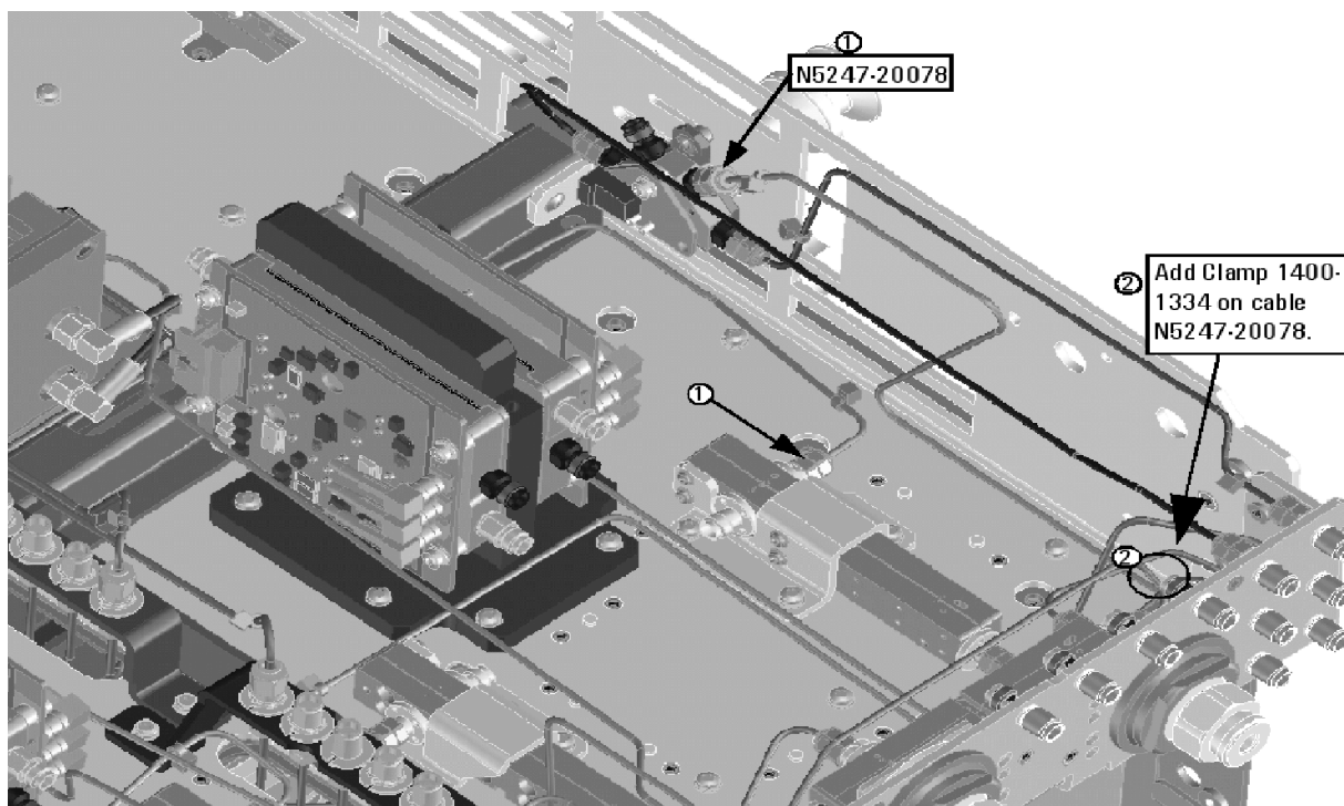
Figure 25 Location of W33 Cable Securing Clamp (1400-1334, N5247-20078)
