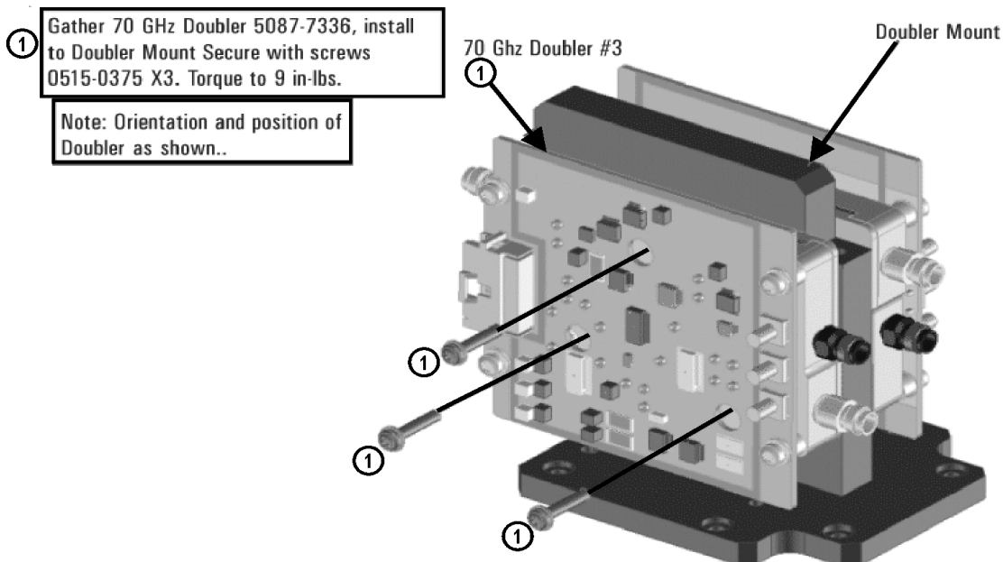
Figure 2 Installing A61 Doubler 3 on the Doubler Mount (0515-0375, 5087-7336)
