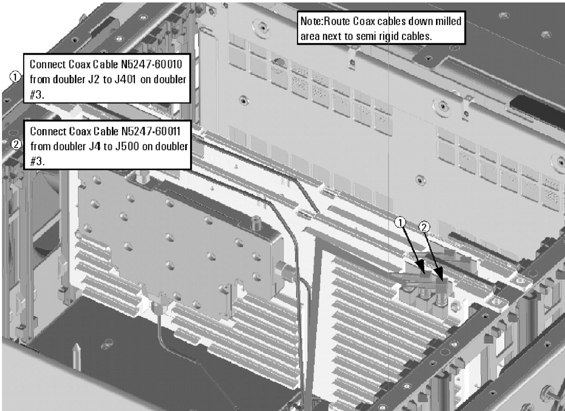
Figure 7 A12 40 GHz Doubler 3 Assembly Cable Installation (N5247-60010, N5247-60011)
