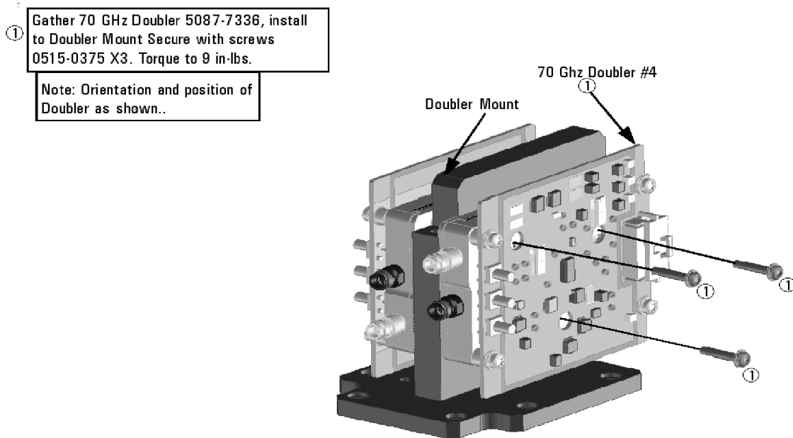
Figure 4 Installing A62 Doubler 4 on the Doubler Mount (0515-0375, 5087-7336)
