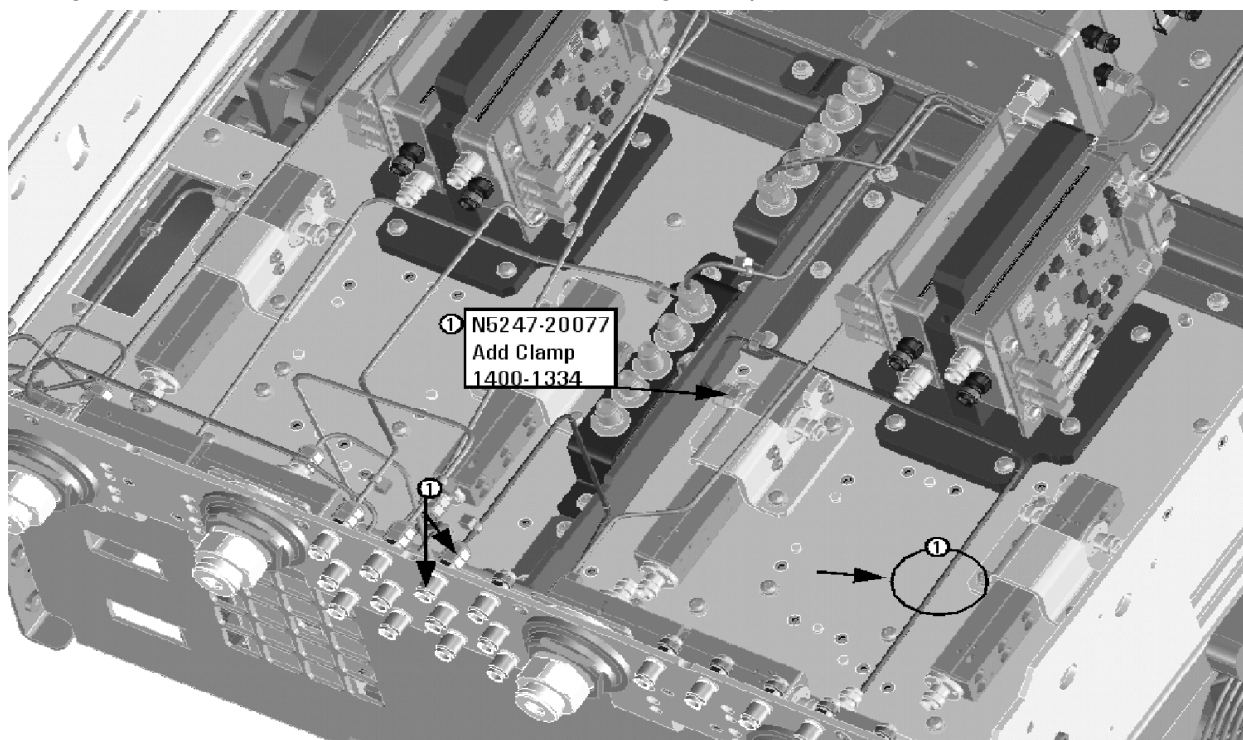
Figure 24 Location of W37 Cable Securing Clamp (1400-1334, N5247-20077)
