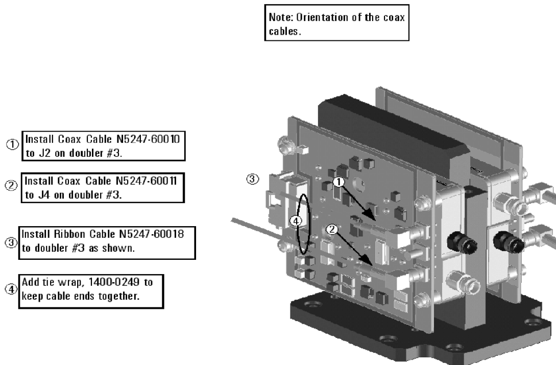
Figure 3 A61 70 GHz Doubler Assembly (1400-0249, N5247-60010, N5247-60011, N5247-60018)
