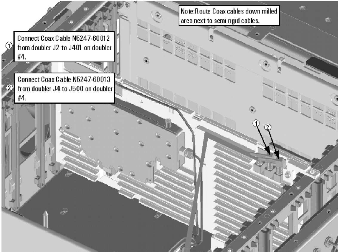
Figure 9 A13 40 GHz Doubler 4 Cable Installation (N5247-60012, N5247-60013)
