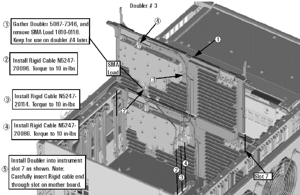
Figure 6 A12 40 GHz Doubler 3 Assembly Installation (1810-0118, 5087-7346, N5247-0086, N5247-20086, N5247-20096, N5247-20114)
