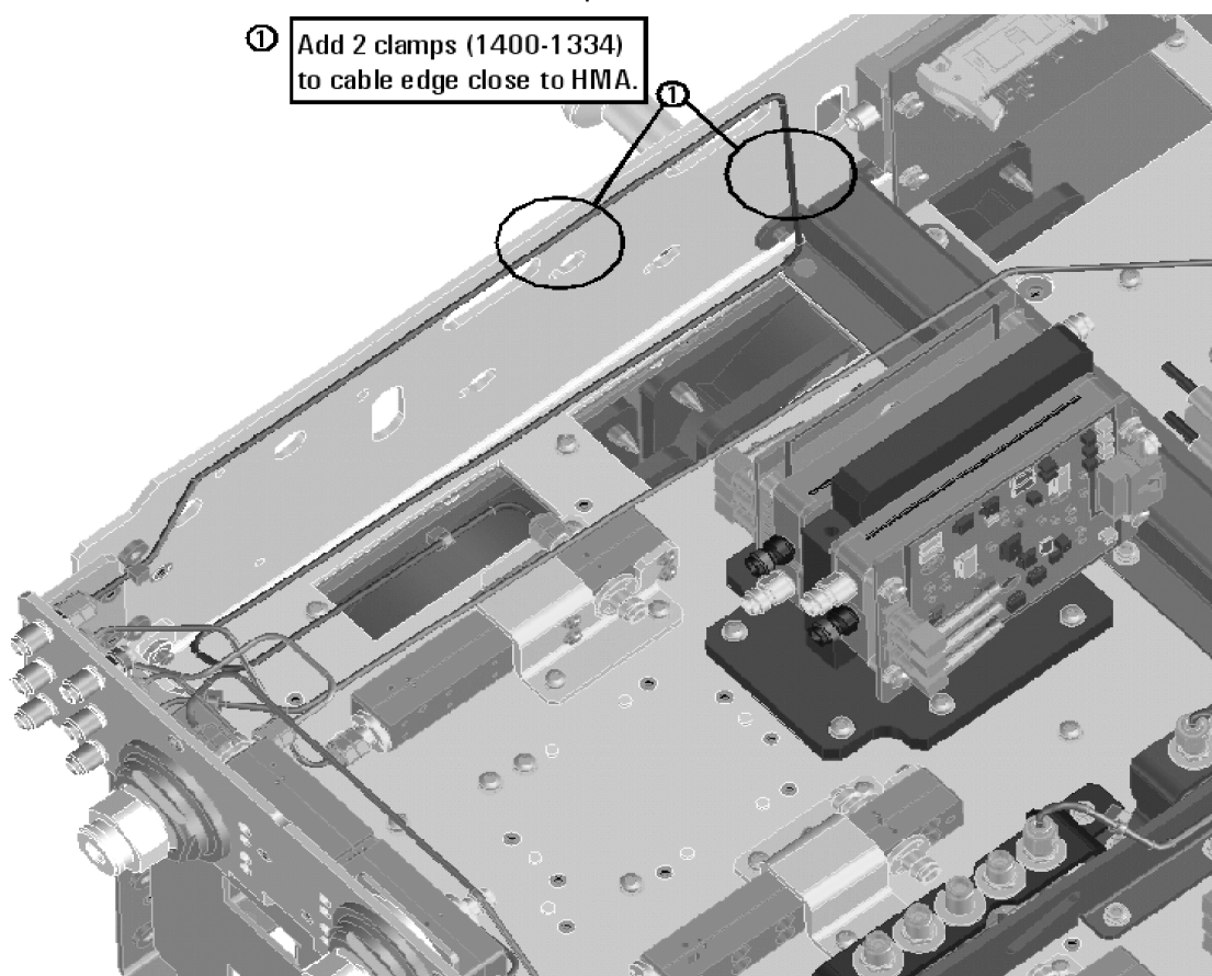
Figure 22 Location of Two Cable Clamps to Secure W45 (1400-1334)
