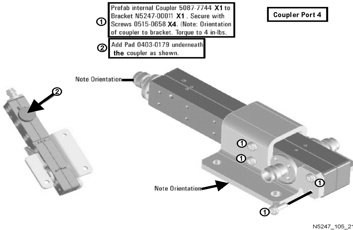
Figure 18 A31 Reference Coupler Assembly (0403-0179, 0515-0658, 5087-7744, N5247-00011)
