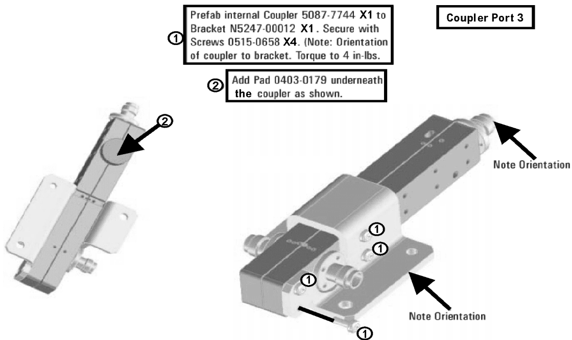
Figure 17 A30 Reference Coupler Assembly (0403-0179, 0515-0658, 5087-7744, N5247-00012)
