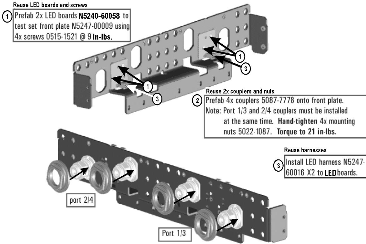
Figure 20-1 LED Board Assemblies and Test Port Coupler Assemblies Installation (0515-1521, 5022-1087, 5087-7778, N5240-60058, N5247-00009, N5247-60016)
