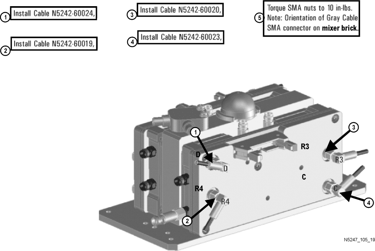
Figure 16 A28 Mixer Brick Cable Installation (N5242-60019, N5242-60020, N5242-60023, N5242-60024)
