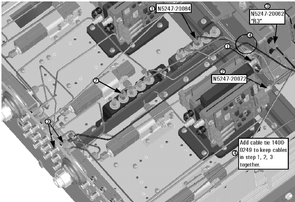
Figure 26 Location of Cable Tie to Secure W14, W18, and W54 Together (1400-0249, N5247-20062, N5247-20072, N5247-20084)
