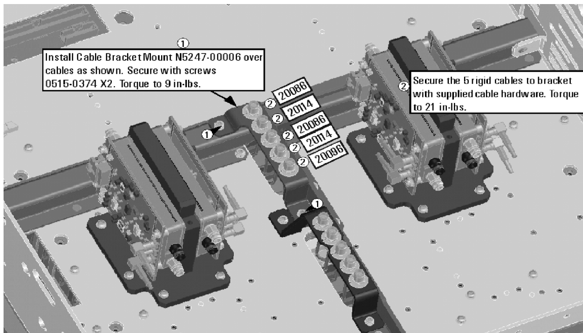
Figure 13 A10 Source 2 Assembly Bracket Installation (0515-0374, N5247-00006)
