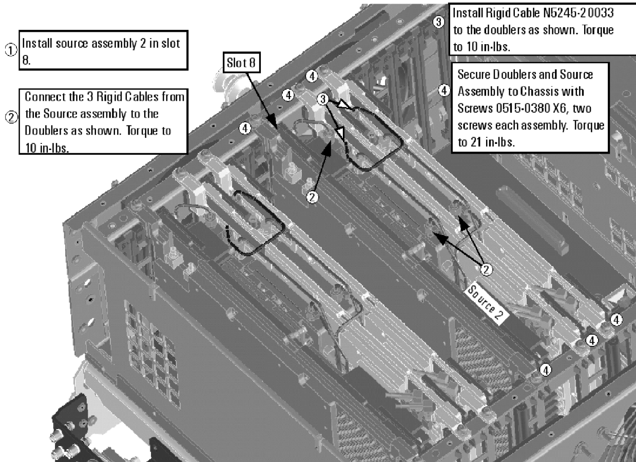
Figure 12 A10 Source 2 Assembly Installation (0515-0380, N5245-20033)
