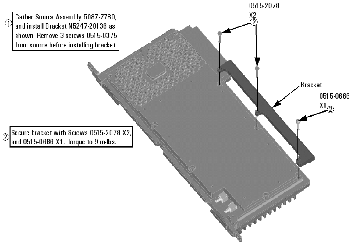
Figure 10 A10 Source 2 Assembly Bracket Installation (0515-0375, 0515-2078, 0515-0666, 5087-7780, N5247-20136)
