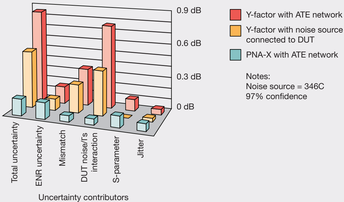
Figure 1. Breakdown of the major contributors to noise figure measurement uncertainty for the Y-factor and cold-source (with source correction) techniques.
