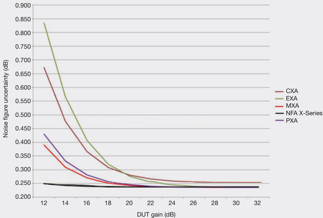
Figure 3. As the gain of a DUT decreases, Y-factor noise figure measurement uncertainty increases; below 20 dB of gain, there are significant differences between the various instrument choices.
