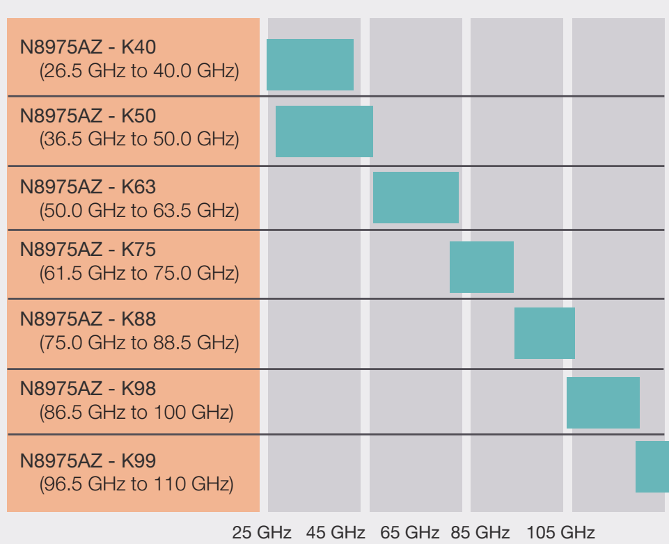
Figure 4. K-Series block downconverter frequency range chart.
